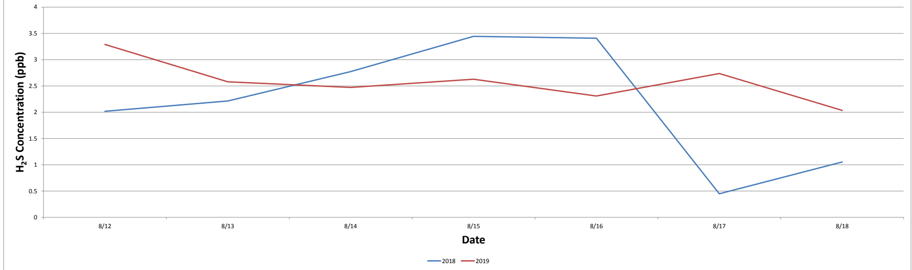
ROX8 Daily Average Comparison for 3rd Week of August in 2018 and 2019
