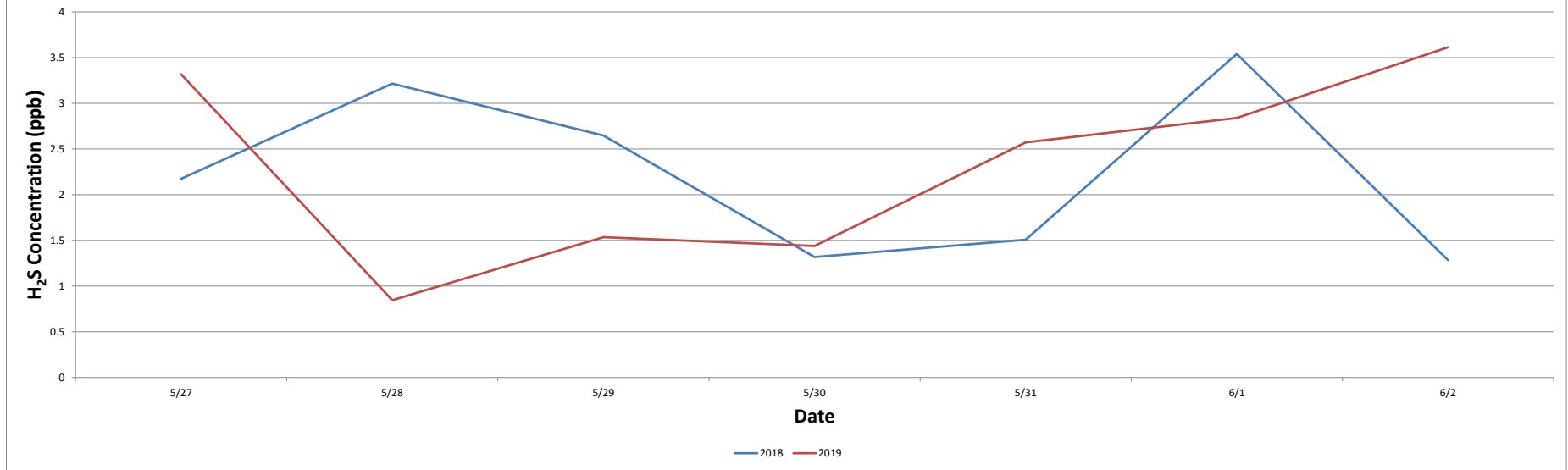
ROX7 Daily Average Comparison for 5th Week of May in 2018 and 2019
