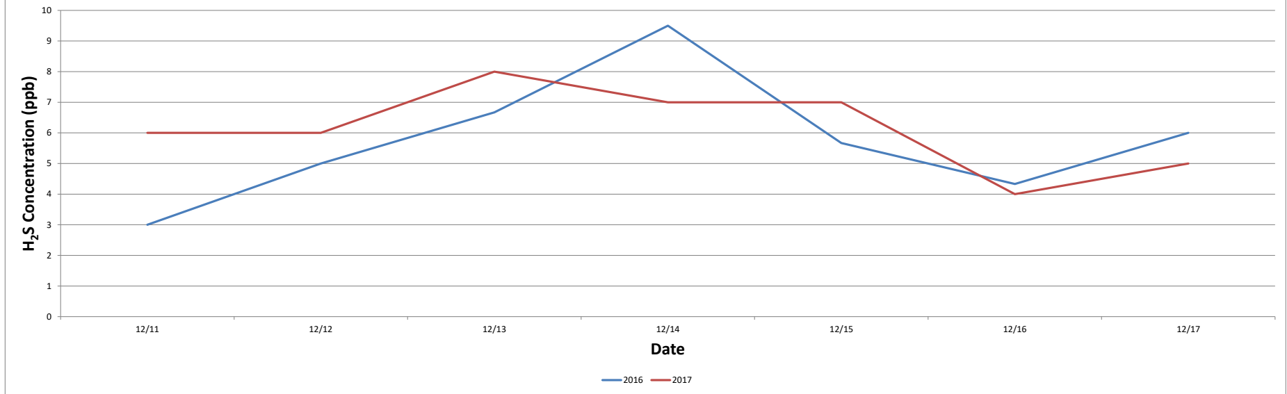
ROX7 Daily Maximum Comparison for 2nd Week of December in 2016 and 2017
