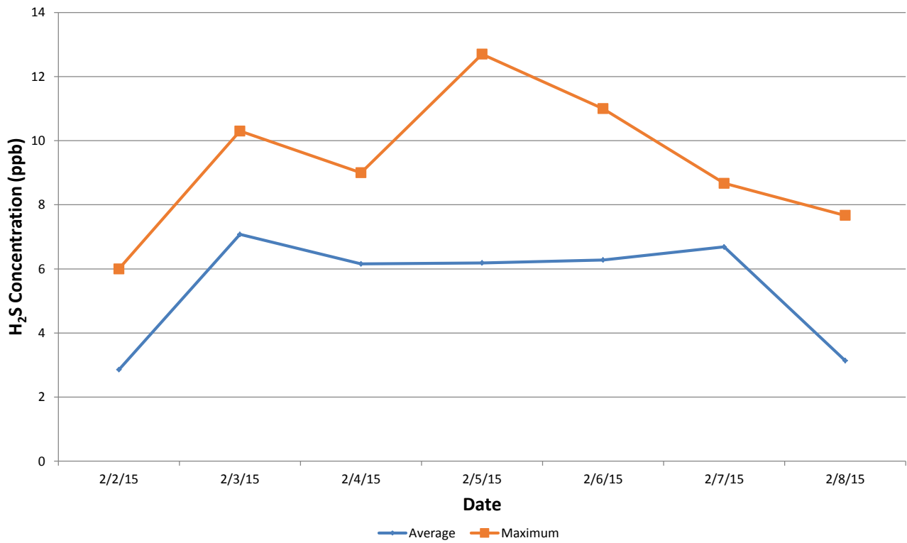
H 2 S Daily Average and Maximum Concentrations at Station #6 in Roxbury, NJ
