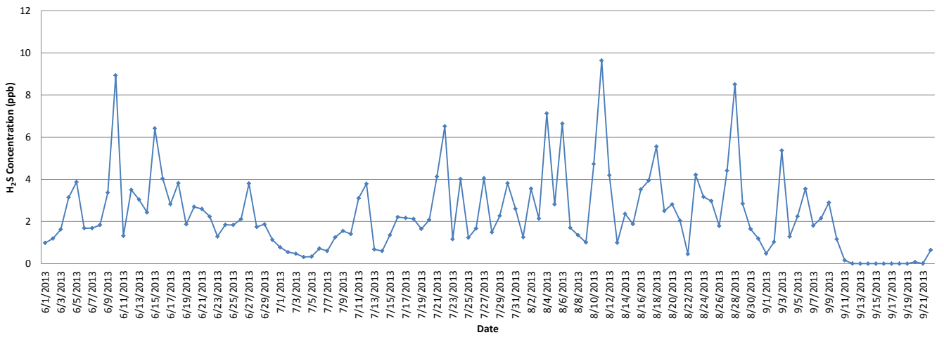
Daily Average Concentration of H 2 S from 6/1/13-9/22/13 @ ROX5
