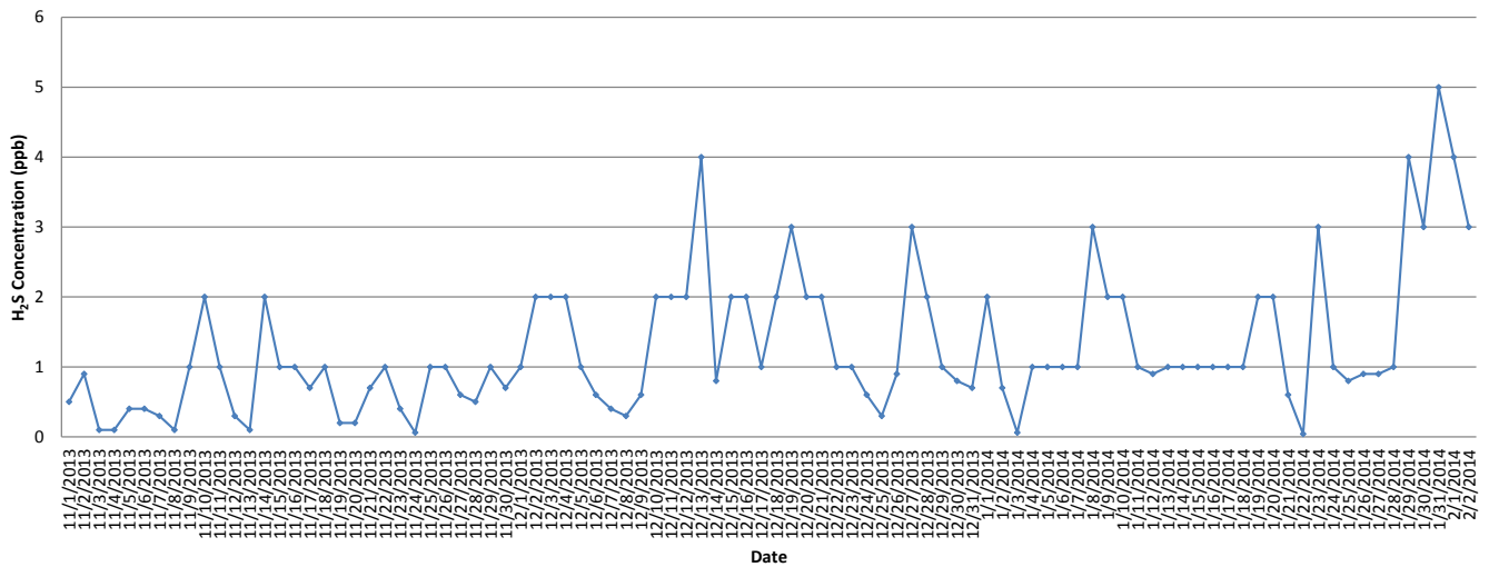
Daily Average Concentration of SO 2 from 11/1/13-2/2/14 @ ROX7
