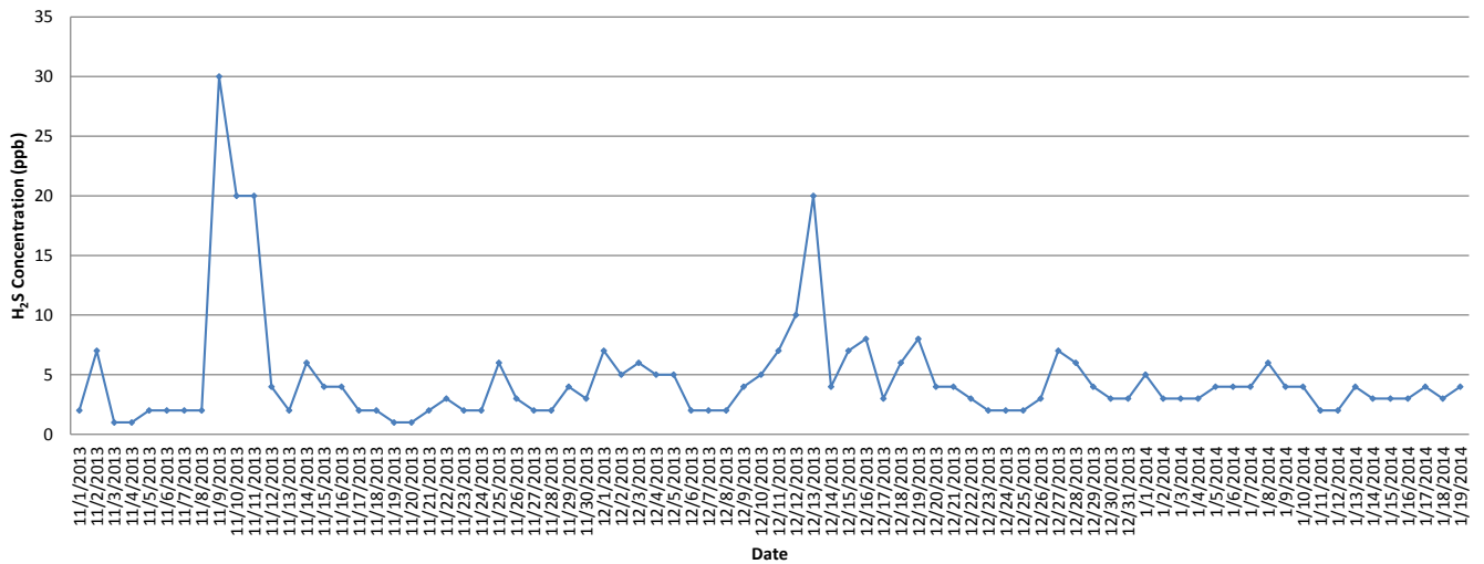
Daily Maximum Concentration of SO 2 from 11/1/13-1/19/14 @ ROX7
