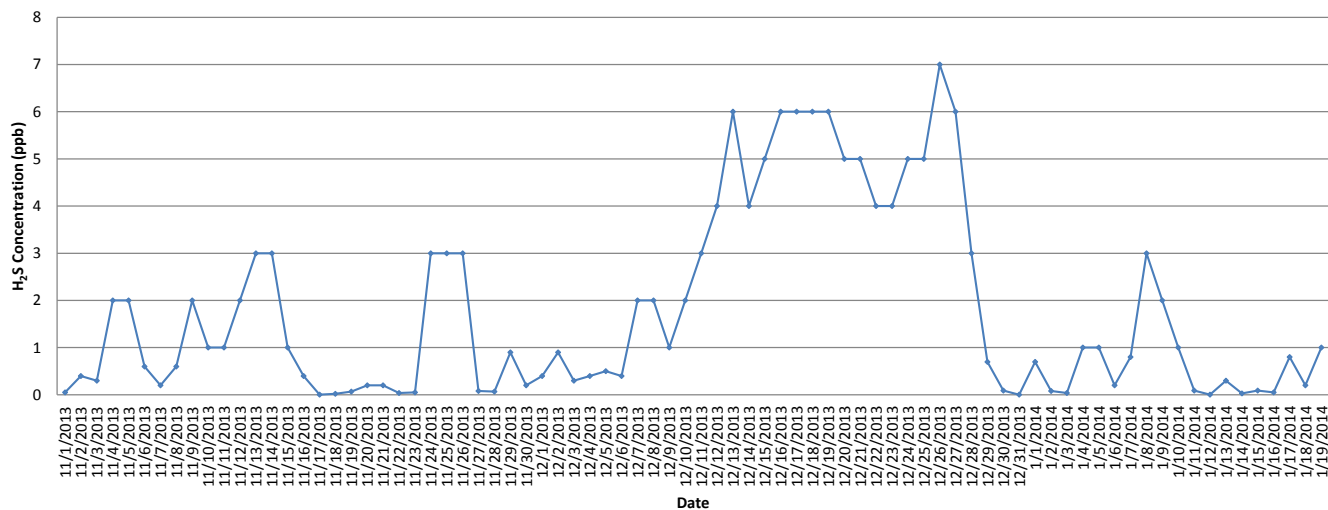
Daily Average Concentration of SO 2 from 11/1/13-1/19/14 @ ROX6
