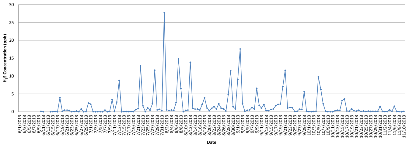
Daily Average Concentration of H 2 S from 6/1/13-11/10/13 @ ROX6
