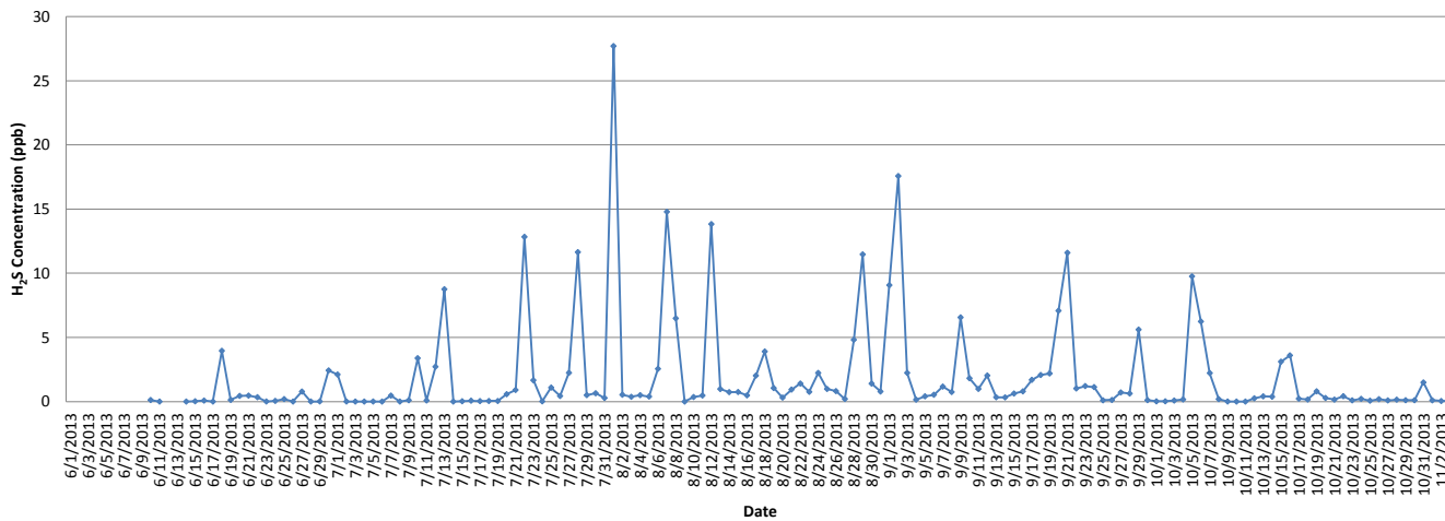
Daily Average Concentration of H 2 S from 6/1/13-11/3/13 @ ROX6
